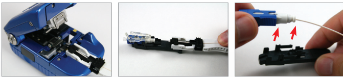
▶ 1 Cutting Fiber ▶ 2 Inserting Fiber ▶ 3 Take Out Connector
